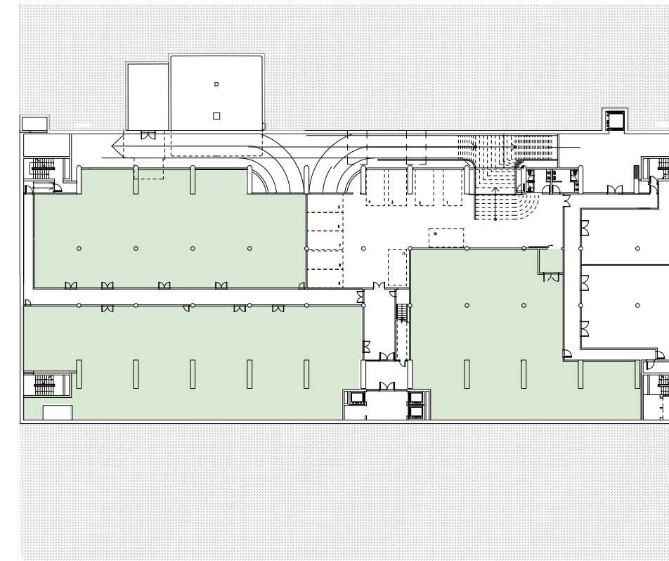
Planta sótano -1 Basement Floor (-1)
